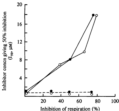
Fig. 5. Dependence of the I_{50} for inhibition by HQNO on the respiration rate. The respiration rate was altered by addition of cyanide (----) or by substrate-limitation (—). The data are taken from Figs 3 and 4. ○, Glucose; ●, NADH.
