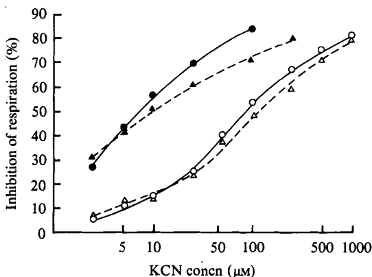
Fig. 2. Inhibition of respiration by cyanide in whole cells and membrane fractions of A. calcoaceticus LMD 79-39. —, Inhibition observed when using whole bacteria harvested after 4.5 h (●) or 8.5 h (○). Identical results were obtained with either glucose or succinate as substrate. ----, Inhibition observed when using membrane fractions from bacteria harvested after 5 h (▲) or 15 h (△). Identical results were obtained when using glucose or NADH as substrate. Only one oxidase (cytochrome o ) was present during the early phase of growth (4.5 or 5 h) but a second oxidase (cytochrome d ) was also present at the later stages of growth (8.5 and 15 h) (see Table 1 and Fig. 1). The uninhibited respiration rates were in the range 150–250 nmol O 2 min -1 (mg dry weight) -1 for whole bacteria, and 250–350 nmol O 2 min -1 (mg protein) -1 for membrane fractions.
