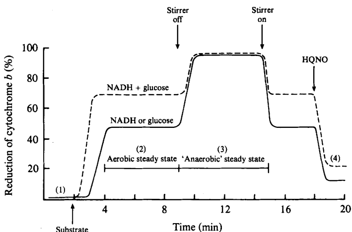
Fig. 6. Reduction of cytochrome b in membranes of A. calcoaceticus LMD 79-39. The reduction of cytochrome b was measured in a 3 ml stirred cuvette in a dual wavelength spectrophotometer using the wavelength pair 560–575 nm; details are given in Methods (the protein concentration was 1.5 \text{ mg ml}^{-1} ). The reduction of cytochrome b is expressed as a percentage of the total that it is reducible with sodium dithionite. (1) In the stirred membrane suspension there was no endogenous respiration and all the cytochrome present (cytochrome b and cytochrome o ) was in the oxidized state. (2) Upon addition of substrate, cytochrome reduction was observed after a lag period during which most of the \text{O}_2 in the stirred cuvette was consumed, leading to the aerobic steady state; the extent of reduction of cytochrome in this state could be adjusted by modifying the aeration rate or by adding low concentrations of HQNO. (3) The stirrer was turned off thus producing the 'anaerobic' steady state. (4) Addition of HQNO during the aerobic steady state led to an immediate fall in the level of reduced cytochrome b . Addition of HQNO in the anaerobic steady state had no effect on the extent of reduction of cytochrome b .
