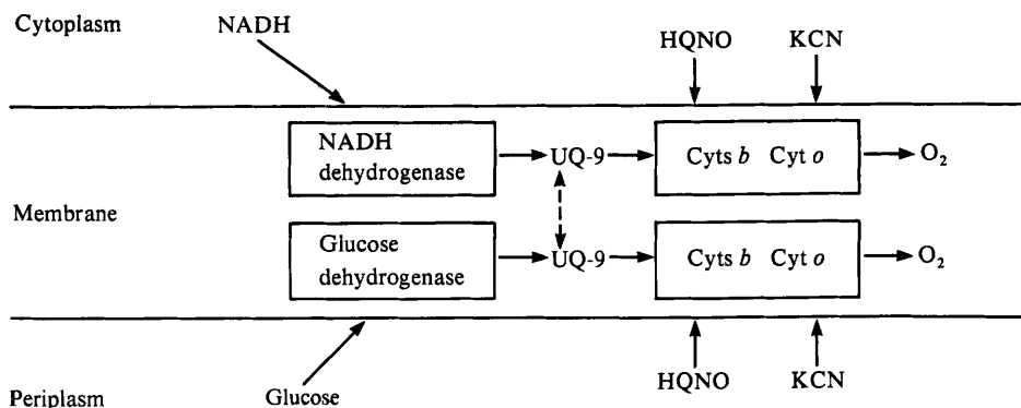
Fig. 7. Oxidation of glucose and NADH in A. calcoaceticus LMD 79-39 grown in conditions of oxygen sufficiency. The components in boxes are firmly membrane-bound. There is no mobile intermediate between the b -type cytochromes and the o -type oxidase. The two dehydrogenases are on opposite sides of the membrane as indicated. The (cyt b , cyt o ) complexes are probably arranged in identical orientations with respect to the membrane, but they differ in their spatial relationships with respect to the two dehydrogenases. The dotted line indicates that in some conditions the ubiquinone pool (UQ-9) mediates interaction between the two kinetically distinct chains for oxidation of NADH and glucose (see text).
