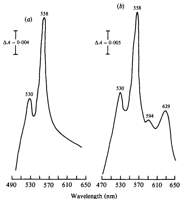
Fig. 1. Effect of growth conditions on cytochrome content of A. calcoaceticus LMD 79-39. The spectra, measured at room temperature are reduced-minus-oxidized difference spectra of the membrane fractions. The reference cuvette contained untreated membranes which were fully oxidized; the test cuvette contained membranes which had been reduced with either glucose, NADH or sodium dithionite; these all gave the same spectrum. (a) Membranes ( 2.5 \text{ mg protein ml}^{-1} ) from bacteria harvested in the early exponential phase of growth (5 h). (b) Membranes ( 3.5 \text{ mg protein ml}^{-1} ) from bacteria harvested in the late exponential phase (12 h).
